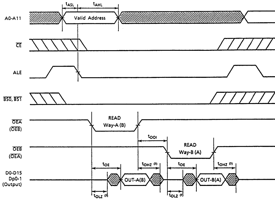
READ CYCLE TIMING 2 ( t_{OOI} TIMING, MODE = V_{IH} )
